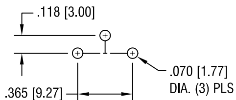
MOUNTING DETAIL
