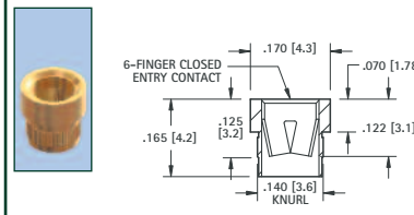
.084 (2.13) - .102 (2.6) PIN - PRESS-FIT
