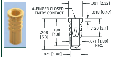
.032 (.81) - .046 (1.17) PIN - PRESS-FIT
