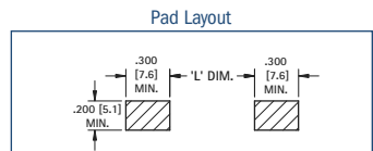
Pad Layout
