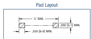
Pad Layout
