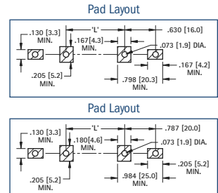
Pad Layout
