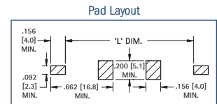
Pad Layout
