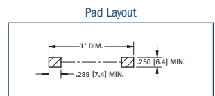
Pad Layout
