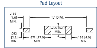
Pad Layout
